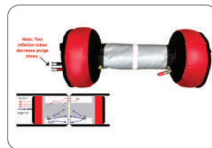
Pipe Purging Equipment
